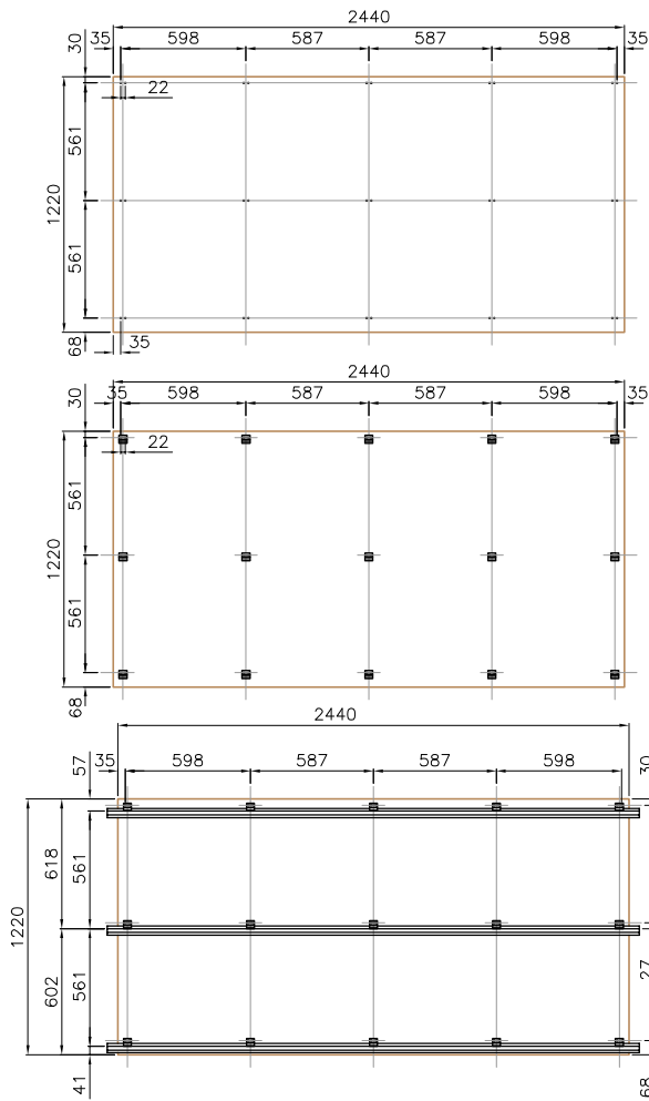
Escala/Scale 1:40
