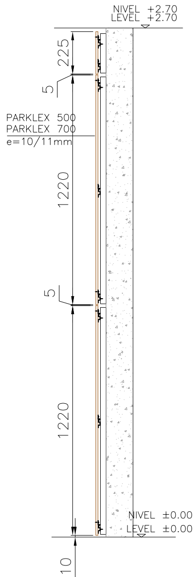
Escala/Scale 1:20
