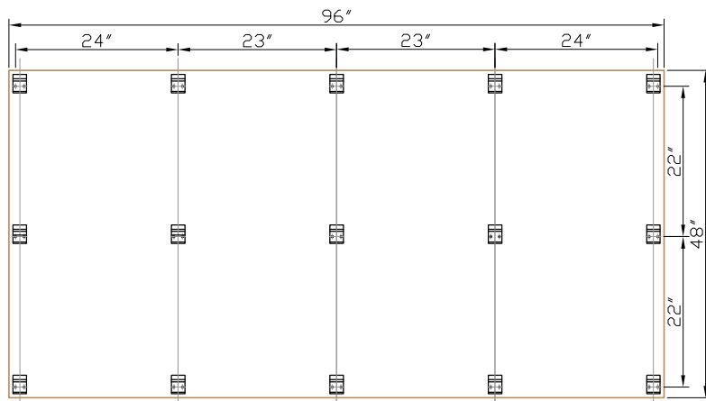
Panel thickness = 3/8"
